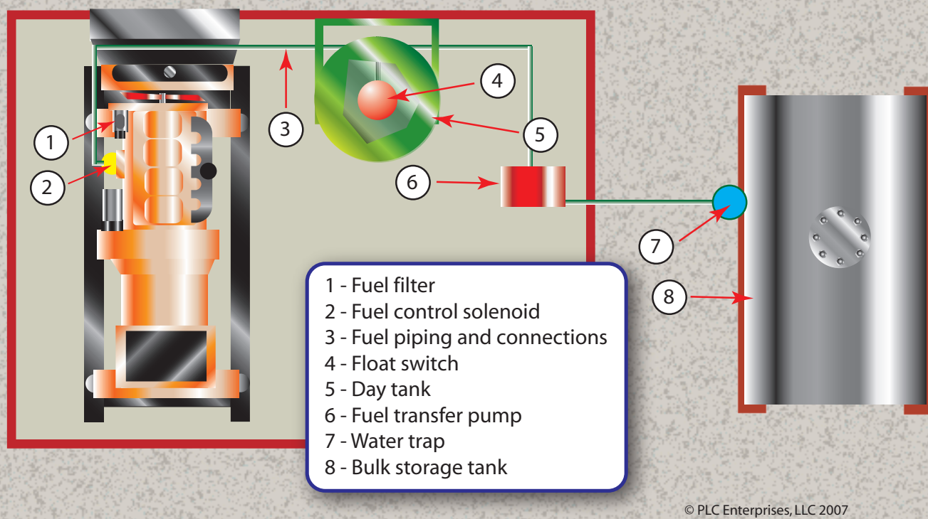
Diagram - Fuel System Maintenance Points
