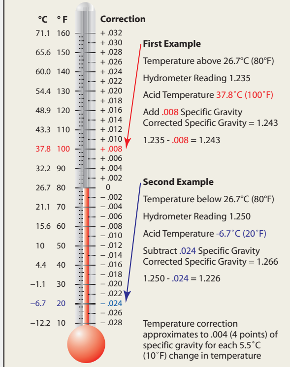
Chart 3- Specific Gravity Temperature Correction
