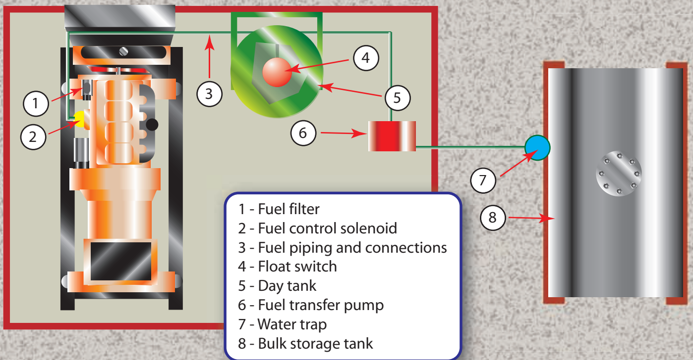
Diagram - Fuel System Maintenance Points
